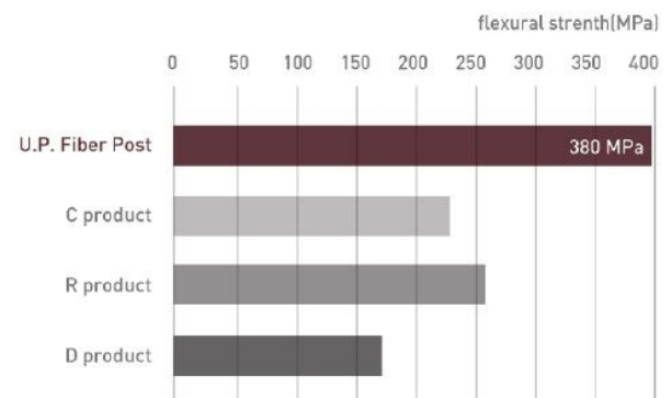
The comparative graph of flexural strength for splinting products
